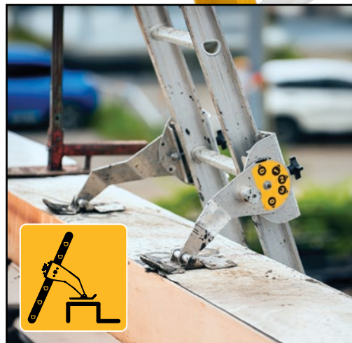
NARROW PARAPET
